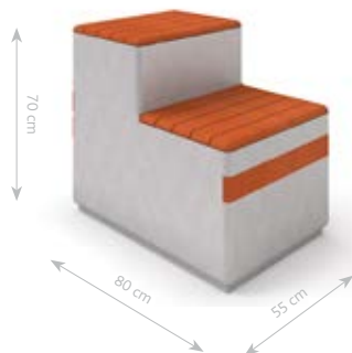
DECO WHITE CONCRETE BENCH 14
