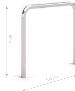
STAINLESS STEEL BICYCLE RACK 22
