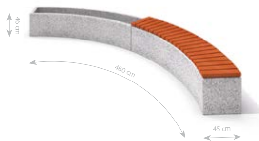
CONCRETE PLANTER SET WITH BENCH 04
