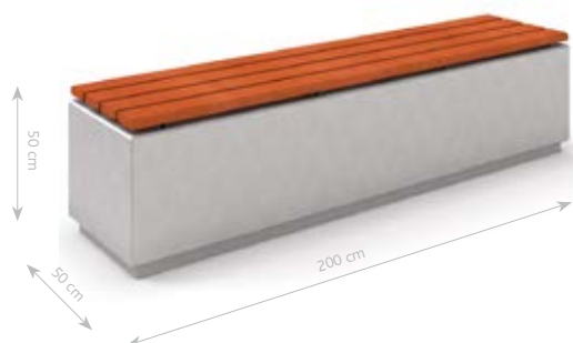
DECO WHITE CONCRETE BENCH 4
