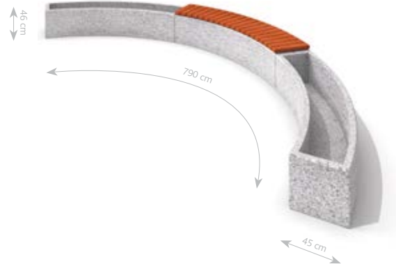
CONCRETE PLANTER SET WITH BENCH 05
