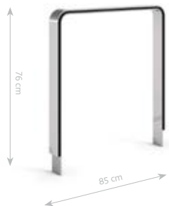
STAINLESS STEEL BICYCLE RACK 24
