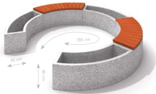
CONCRETE PLANTER SET WITH BENCH 02
