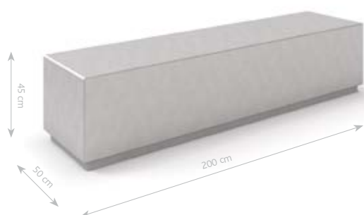
DECO WHITE CONCRETE BENCH 5
