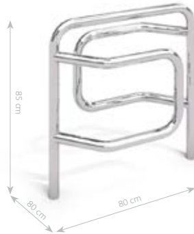
STAINLESS STEEL BICYCLE RACK 09
