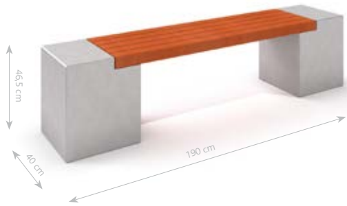
DECO WHITE CONCRETE BENCH 12
